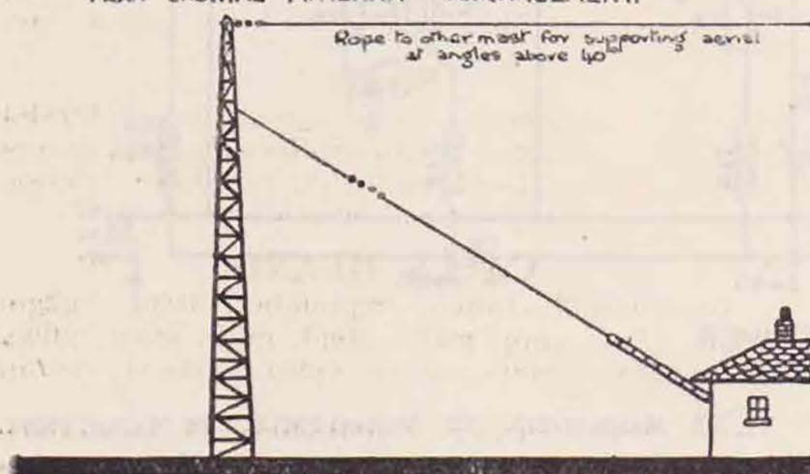
PLAN SHOWING ANTENNA ARRANGEMENT.
